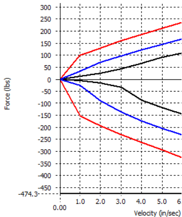
SAMPLE LOW/MID/HI RANGE BLEED ADJUSTMENT INFLUENCE ON DAMPER CURVE
